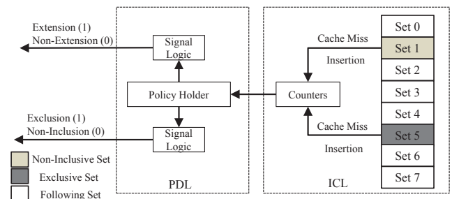
Figure 6. High-level block diagram for mode selection.
