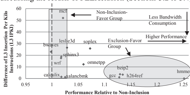
(a) L2:512KB, L3:1MB (1:2 ratio)
