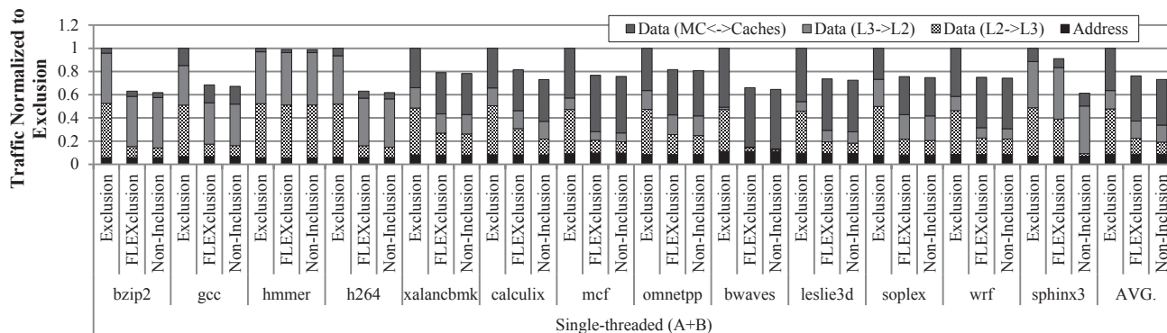
Figure 16. Traffic breakdown for single-threaded workloads (A+B).
