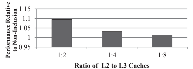
Figure 3. Performance of non-inclusive and exclusive LLCs varying the LLC size for SPEC2K6 benchmarks.
