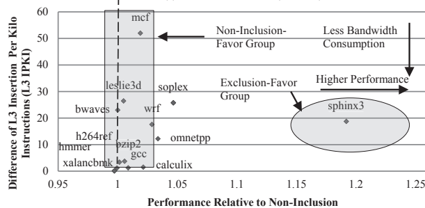
(b) L2:512KB, L3:4MB (1:8 ratio)
