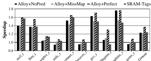
Figure 6: Speedup with Alloy Cache.
