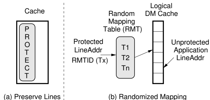
Fig. 3. Prior solutions (a) preservation-based (b) randomization-based
